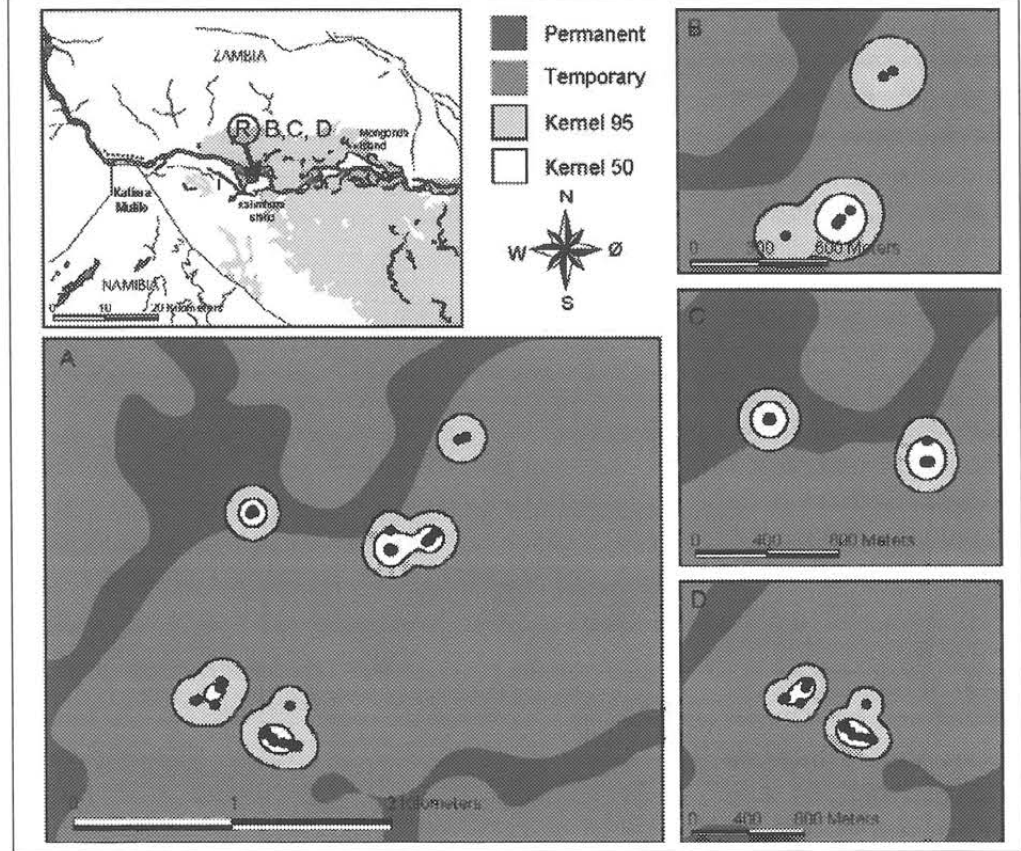
Figure 3. Kernel home ranges of individual radio tagged threespot tilapia ( n = 6 ) in the Zambezi River in 2000 and 2001 during a) the entire study period, b) low water only, c) rising water only, and d) high water only (figure d is lacking for the fish not recorded during the high water period). Dots show fish positions during tracking, and the contours of home ranges refer to two different levels of probability (95 and 50%). Landscape contours refer to permanent and temporary water covered areas. Upper left figure indicates where in the Zambezi River the fish were released (R) and where home ranges were recorded. Individual fish number corresponds to the numbers in table 1.
